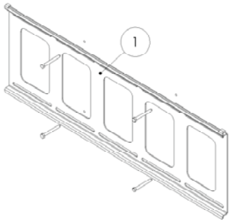
Step 2: Mounting the wall plate (Lag screws are not included)
